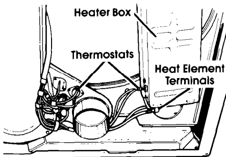
ELECTRIC DRYERS
